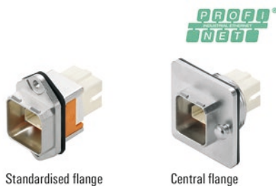
Standardised flange
